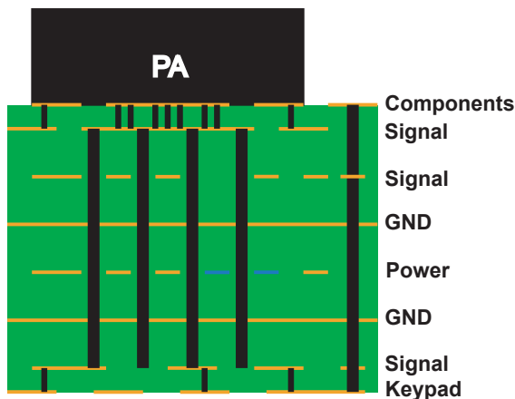
Figure 5: Example of PCB Stack with Microvias on Top and Bottom Layers, Buried Vias From Layers 2 to 7, and through Vias from Layers 1 to 8.
