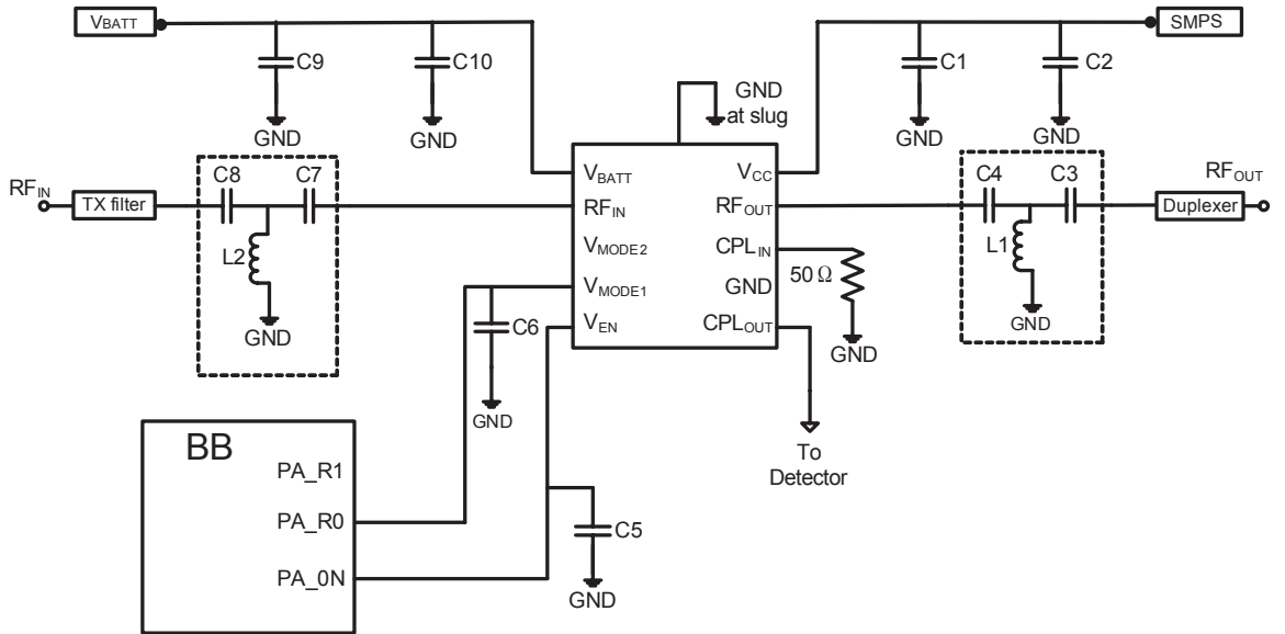
Figure 7: Typical Application Schematic
