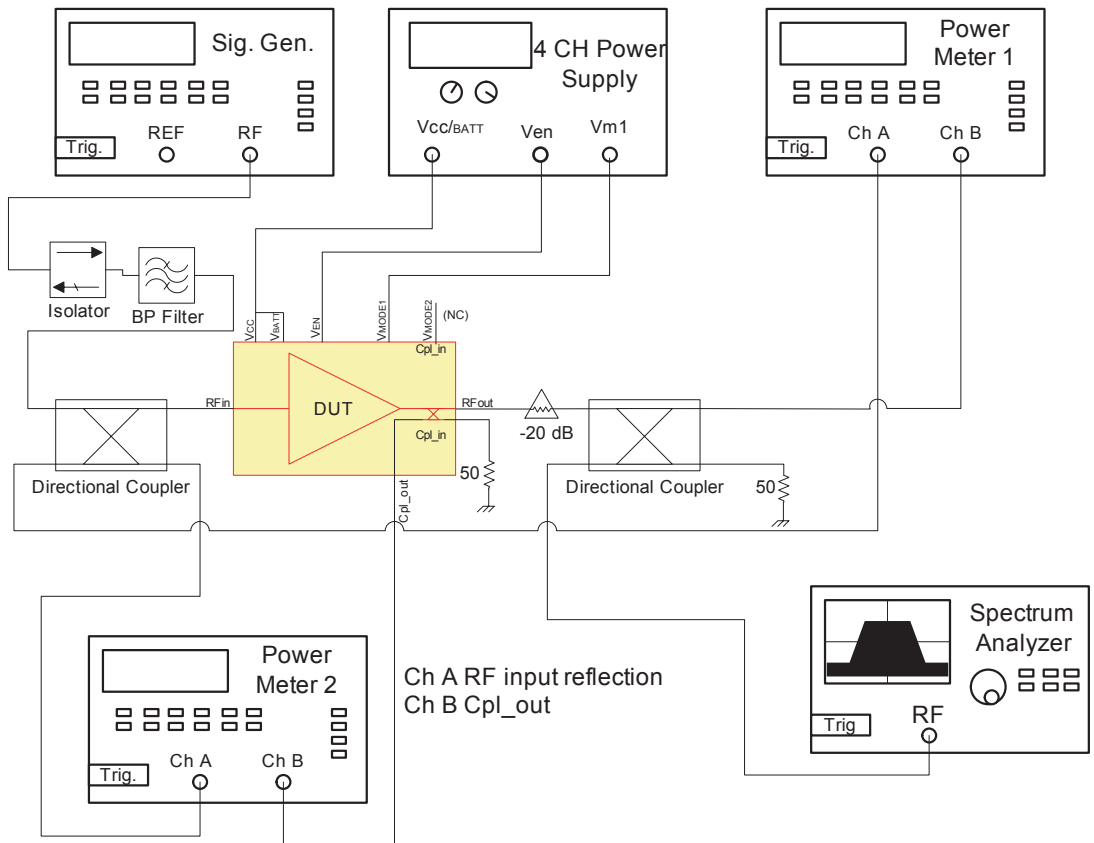
Figure 2: Test Setup Diagram 1
