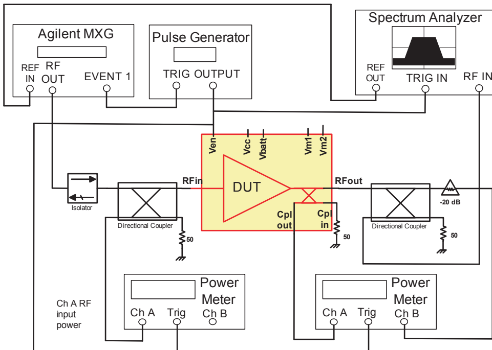
Figure 3: Test Setup Diagram 2
