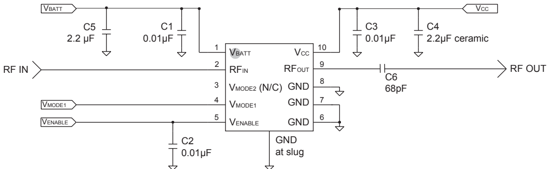
Figure 1: Application Schematic
