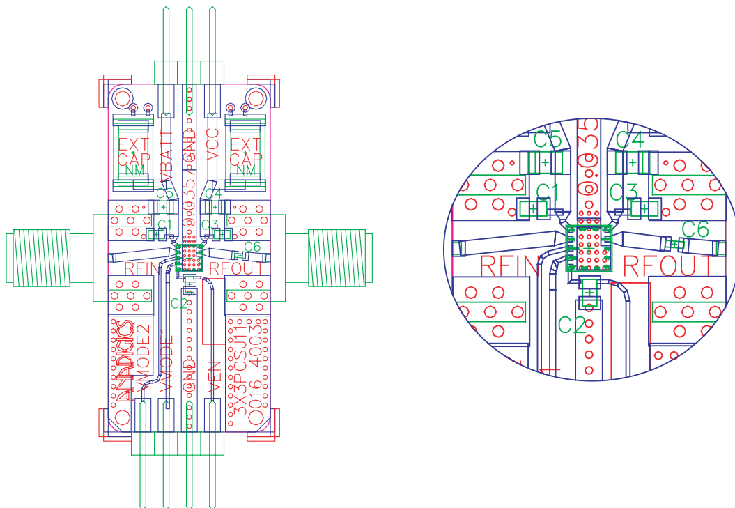
Figure 2: Evaluation Board Layout
