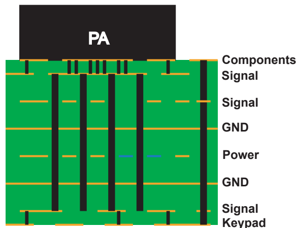
Figure 5: Example of PCB Stack-up with Microvias from Top to Bottom Layers, Buried Vias From Layers 2 to 7, and through Vias from Layer 7
