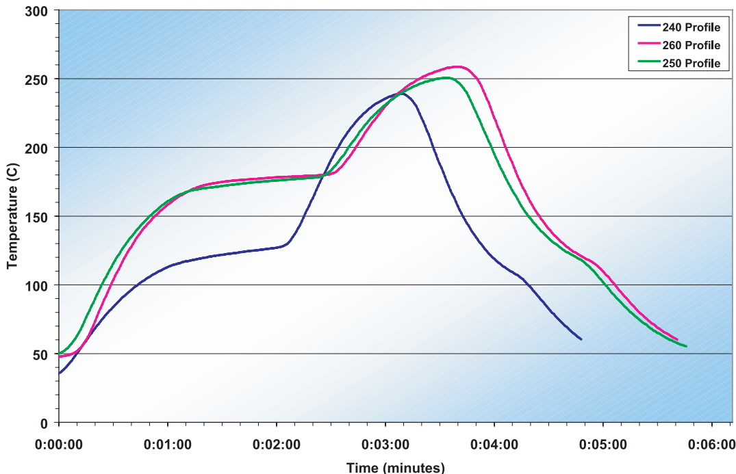
Figure 6: Comparison of High Temperature Reflow Profiles
